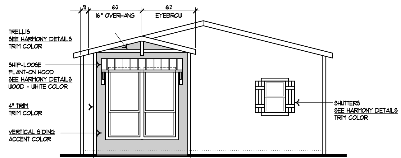
OPTION FRONT ENDWALL
