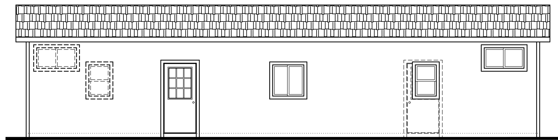
4" FLAT WINDOW AND DOOR TRIM THROUGHOUT. REAR SIDEWALL
