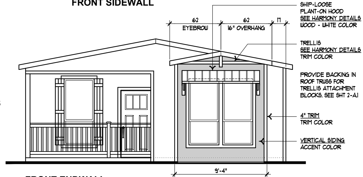
FRONT ENDWALL
