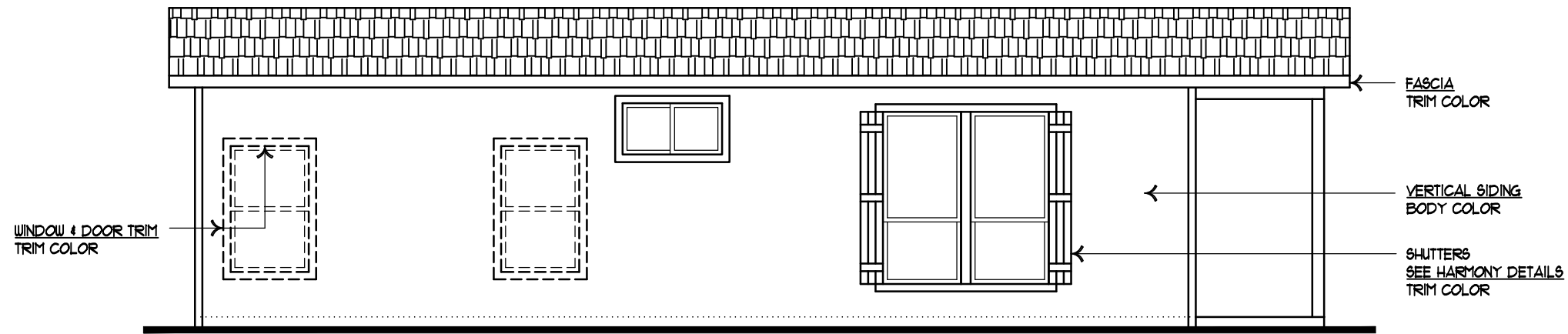
FRONT SIDEWALL
